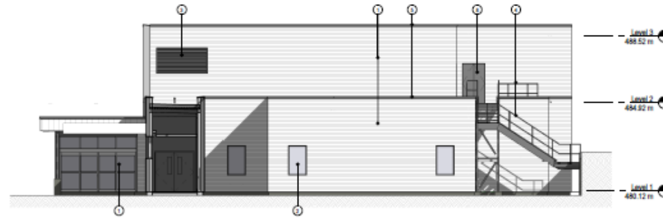
4 SOUTH ELEVATION A201 1:100
